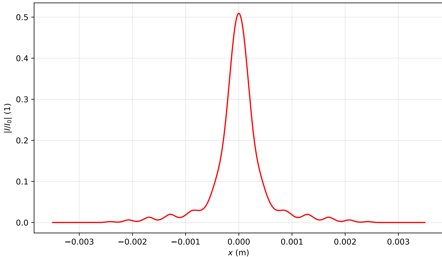
Intensity profile I(x, y = 0, z = 2.707)/I_0 , \text{Pin}=3.0\text{Pcr} , artificial time
